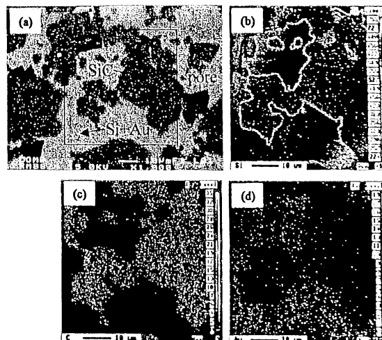
[(b)-Si, (c)-C and (d)-Au] the element distribution image in SiC/Si/Au=55/40/5+PSS10(wt.%).
