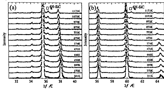
Fig. 5 Temperature dependence of XRD pattern of SiC/Si/Au=55/40/5+PSS10(wt%) (a) 2\theta=31-41^\circ (b) 2\theta=55-65^\circ .
